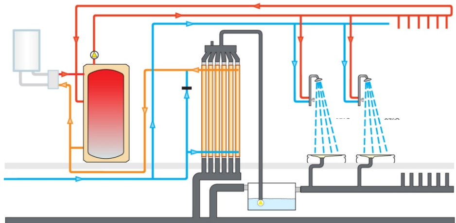
The Recoh ® -multivert, installed in a building where the equipment room is situated on the ground floor and the showers on the upper floors.
